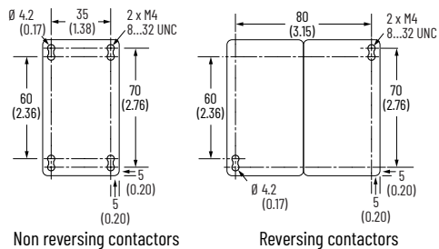
40...65 A Contactors
