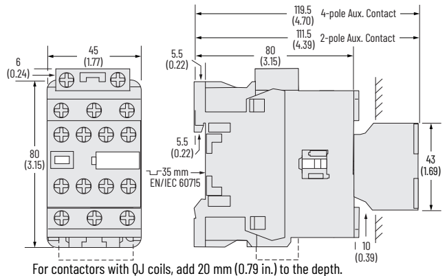
Figure 48 - 100-E26...100-E38 4-Pole Contactors with Standard Coils and Front-mounted Auxiliary Contact
