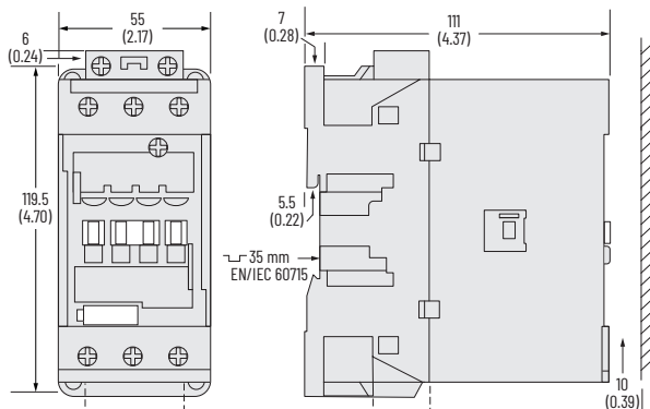
Figure 58 - 100-E40...100-E65 3-Pole Contactors with Front-mounted Auxiliary Contact
